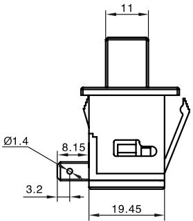
PS9-Z1-B (B型按鈕 Plunger type B )
